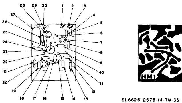
Figure 8-12. 1.0-MHz harmonic marker printed circuit assembly.
