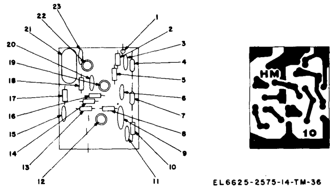
Figure 8-13. 10.0-MHz harmonic marker printed circuit assembly.
