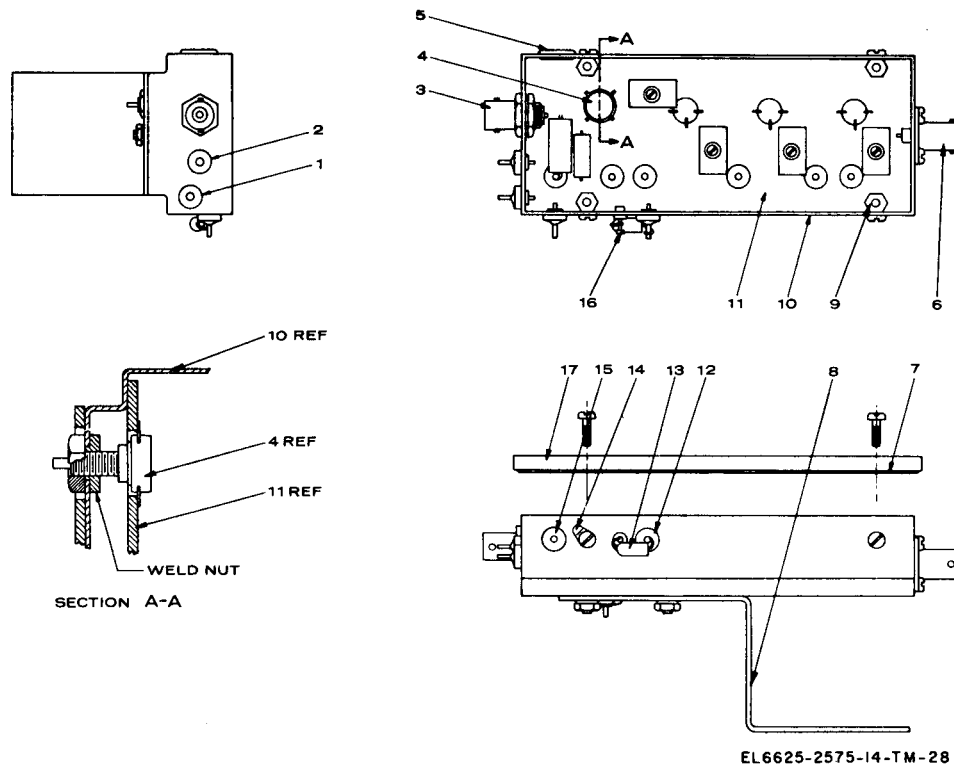
Figure 8-5. Video amplifier assembly.
